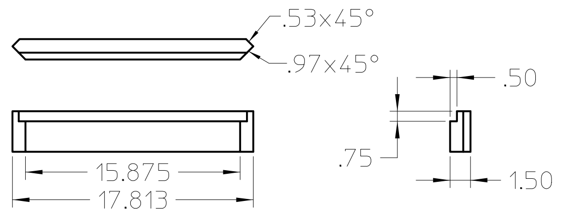
SIDE RAIL (2 reqd)
