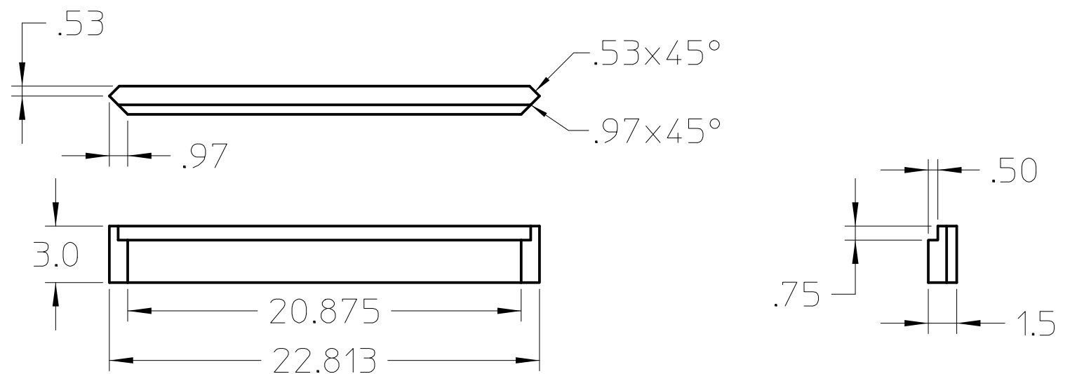
FRONT RAIL (2 reqd)
